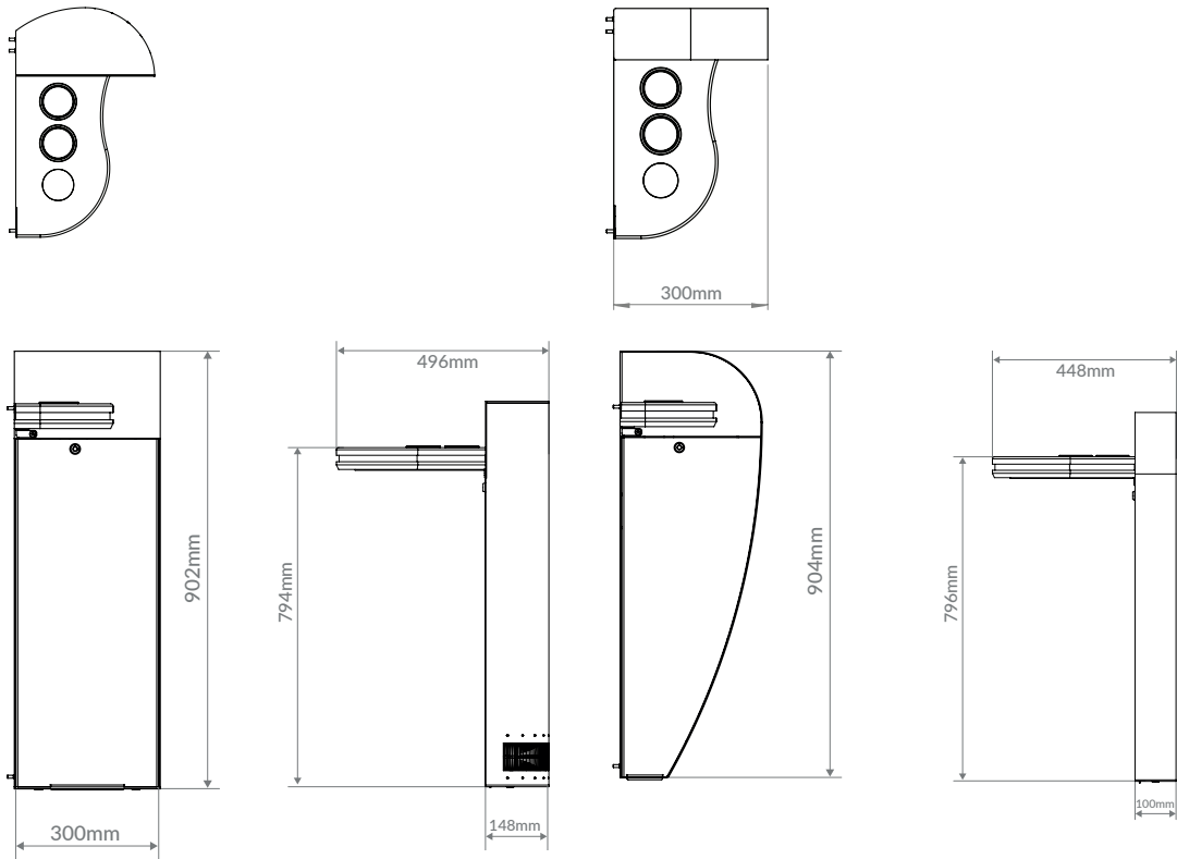
Wedge Assembly
